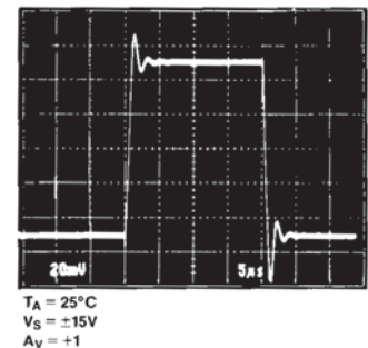
TPC 24. Small-Signal Transient Response C_{LOAD} = 1 \text{ nF}
