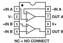
8-Lead SO (S-Suffix)
