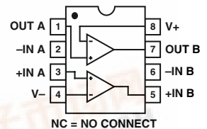
8-Lead HERMETIC DIP (Z-Suffix)
