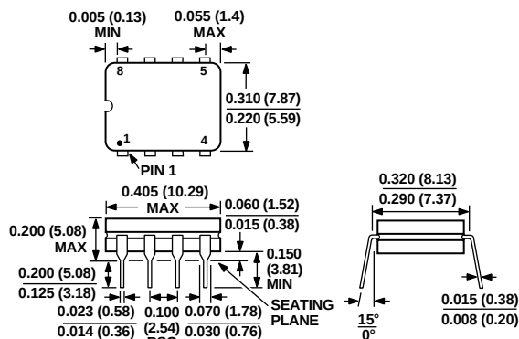
8-Lead Cerdip (Q-8)
