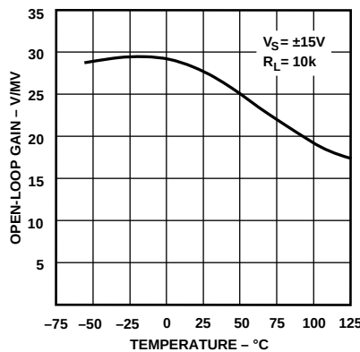
Figure 8. Open-Loop Gain (V/mV)
