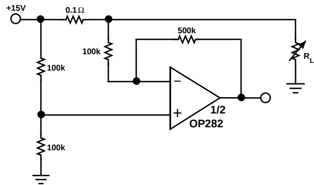
Figure 1. Phase Inversion
