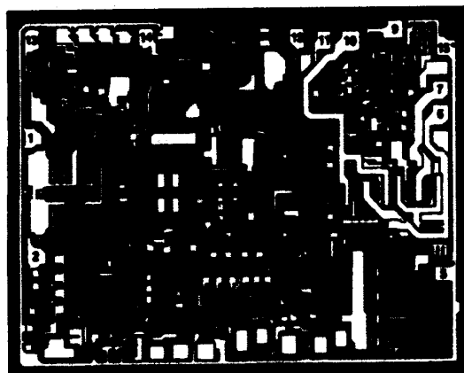
DIE SIZE 0.149 x 0.111 inch, 16,539 sq. mils (3.78 x 2.82 mm, 10.66 sq. mm)
