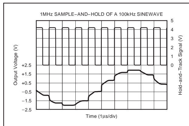
Figure 46. 1MHz Sample-and-Hold of a 100kHz Sine Wave
