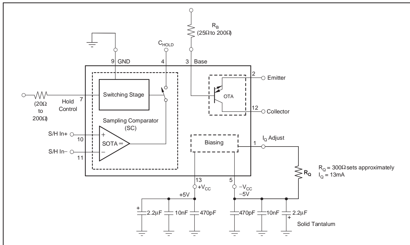
Figure 39. Basic Connections
