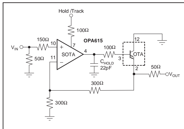
Figure 45. Sample-and-Hold Amplifier
