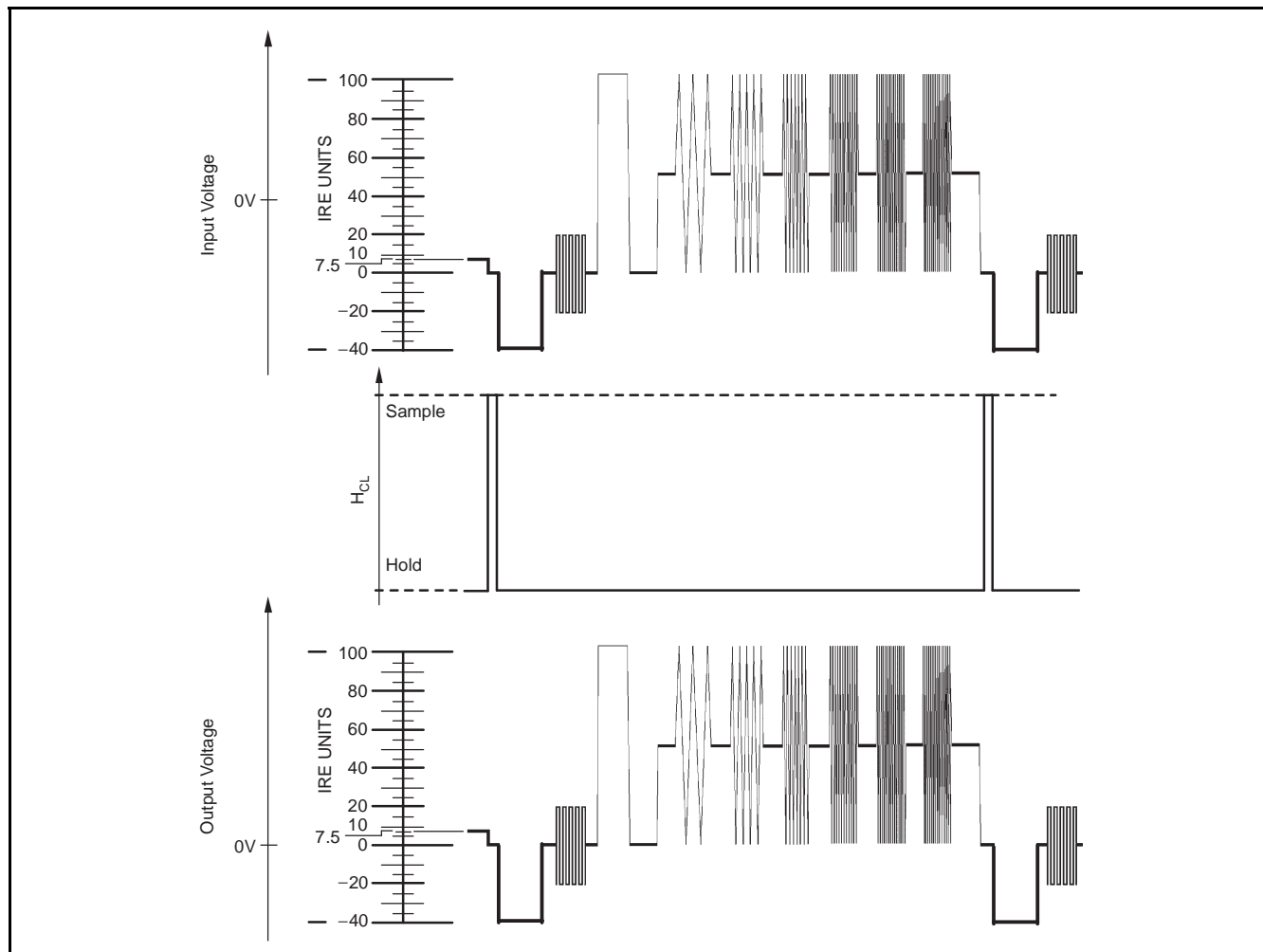
Figure 43. DC-Restore Timing
