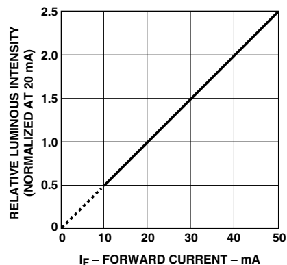
Figure 4. Amber, red relative luminous intensity vs. forward current.
