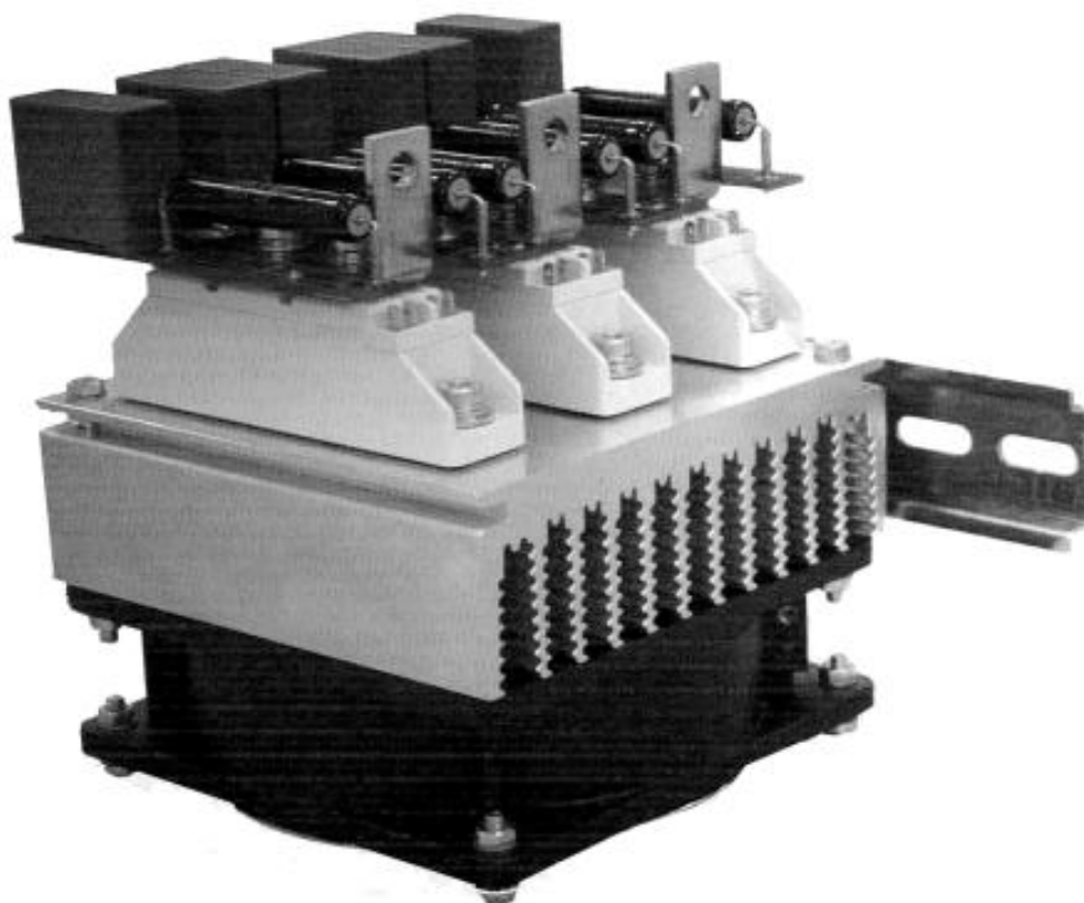
1. Application example using P 23, fan SKF 3 and 3x SEMIPACK 1 modules to give a three phase bridge rectifier
