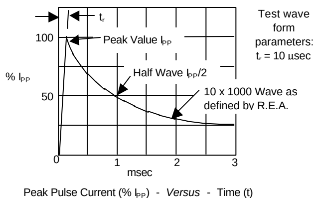
Figure 2 - Pulse Waveform
