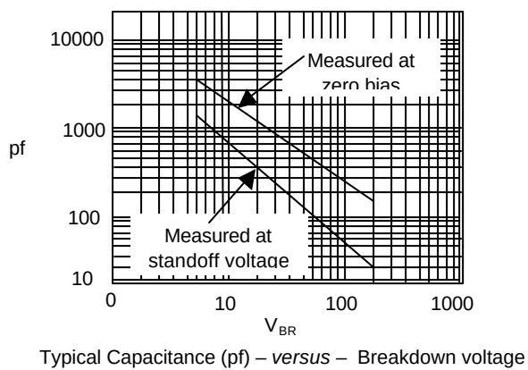
Figure 3 - Typical Capacitance
