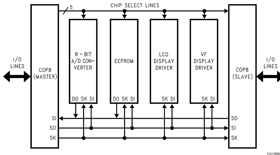
FIGURE 29. MICROWIRE/PLUS Application
