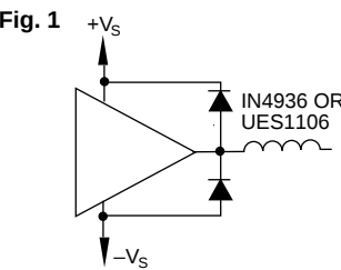
PROTECTION, INDUCTIVE LOAD
