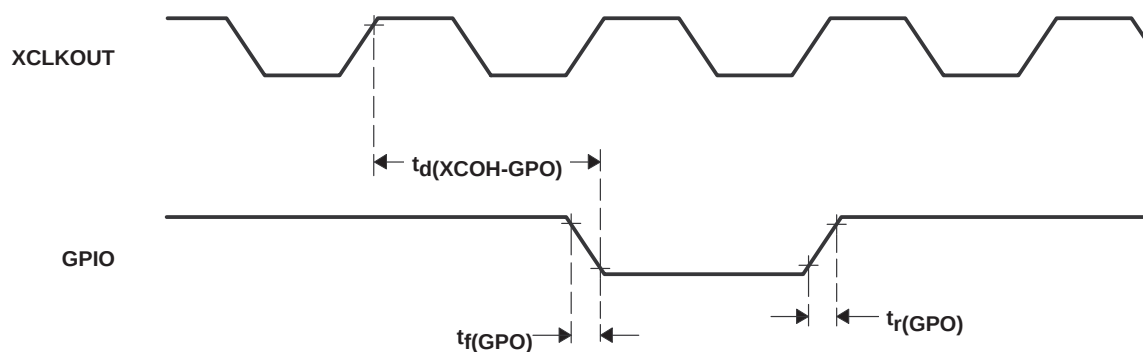
Figure 6-22. General-Purpose Output Timing
