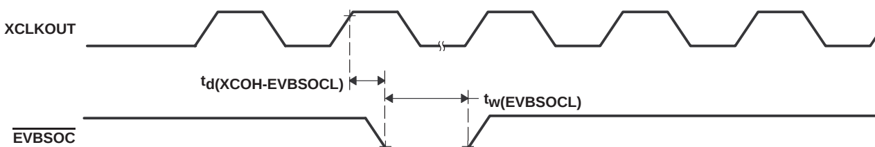
Figure 6–20. \overline{\text{EVBSOC}} Timing
