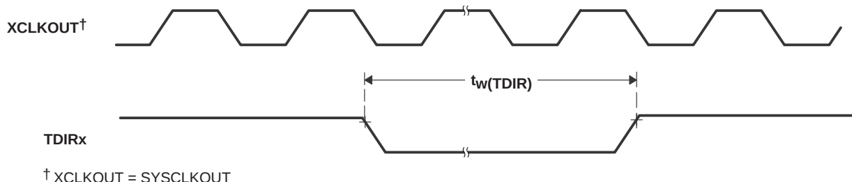
Figure 6–18. TDIRx Timing
