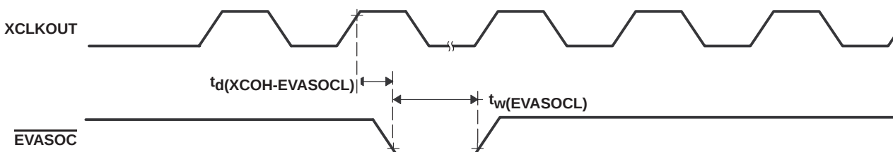
Figure 6–19. \overline{\text{EVASOC}} Timing
