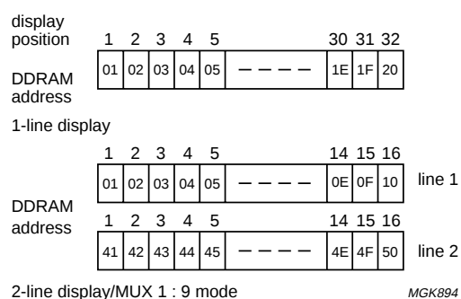
Fig.4 DDRAM to display mapping; left shift: (For 1 \times 32 only as long as 4F and 00 positions are not on display simultaneously).
