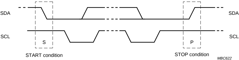
Fig.20 Definition of START and STOP conditions.
