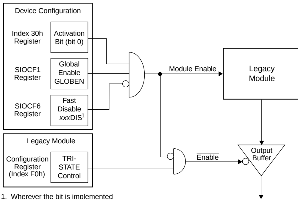
Figure 6. Control of Floating Legacy Module Pins
