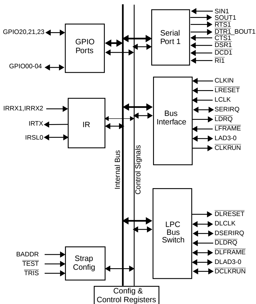
Figure 3. PC87382 Detailed Block Diagram
