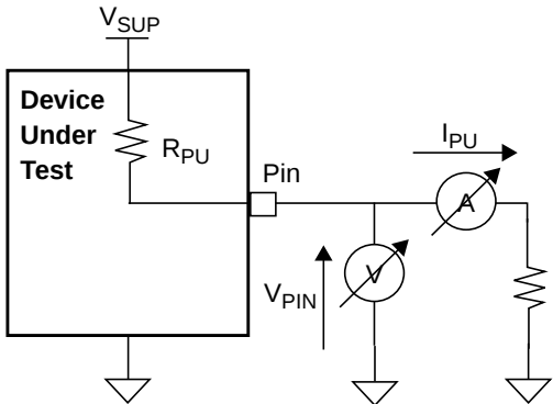
Pull-Up Resistor Test Circuit
