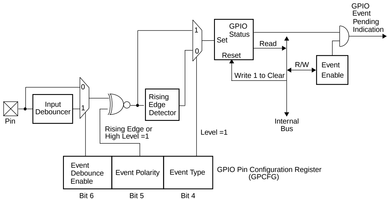
Figure 10. Event Detection
