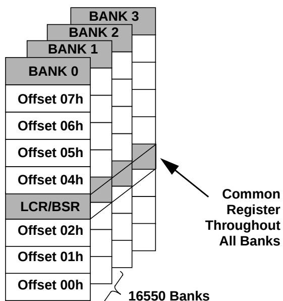
Figure 12. Register Bank Architecture
