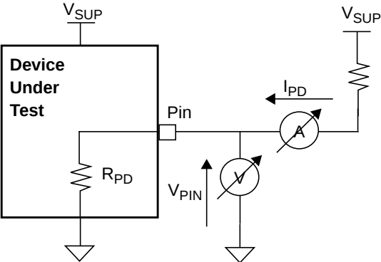
Pull-Down Resistor Test Circuit
