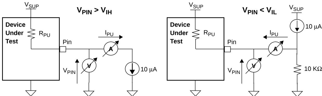
Figure 15. Internal Pull-Down Resistor for Straps, T A = 0°C to 70°C, V SUP = 3.3V
