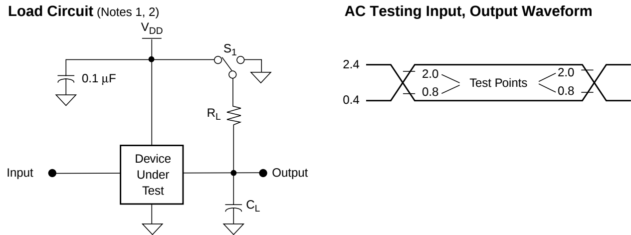
Figure 16. AC Test Conditions, TA = 0 °C to 70 °C, VDD = 3.3 V ±10%
