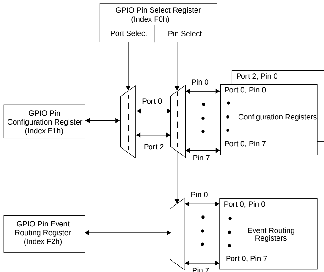
Figure 7. Organization of GPIO Pin Registers
