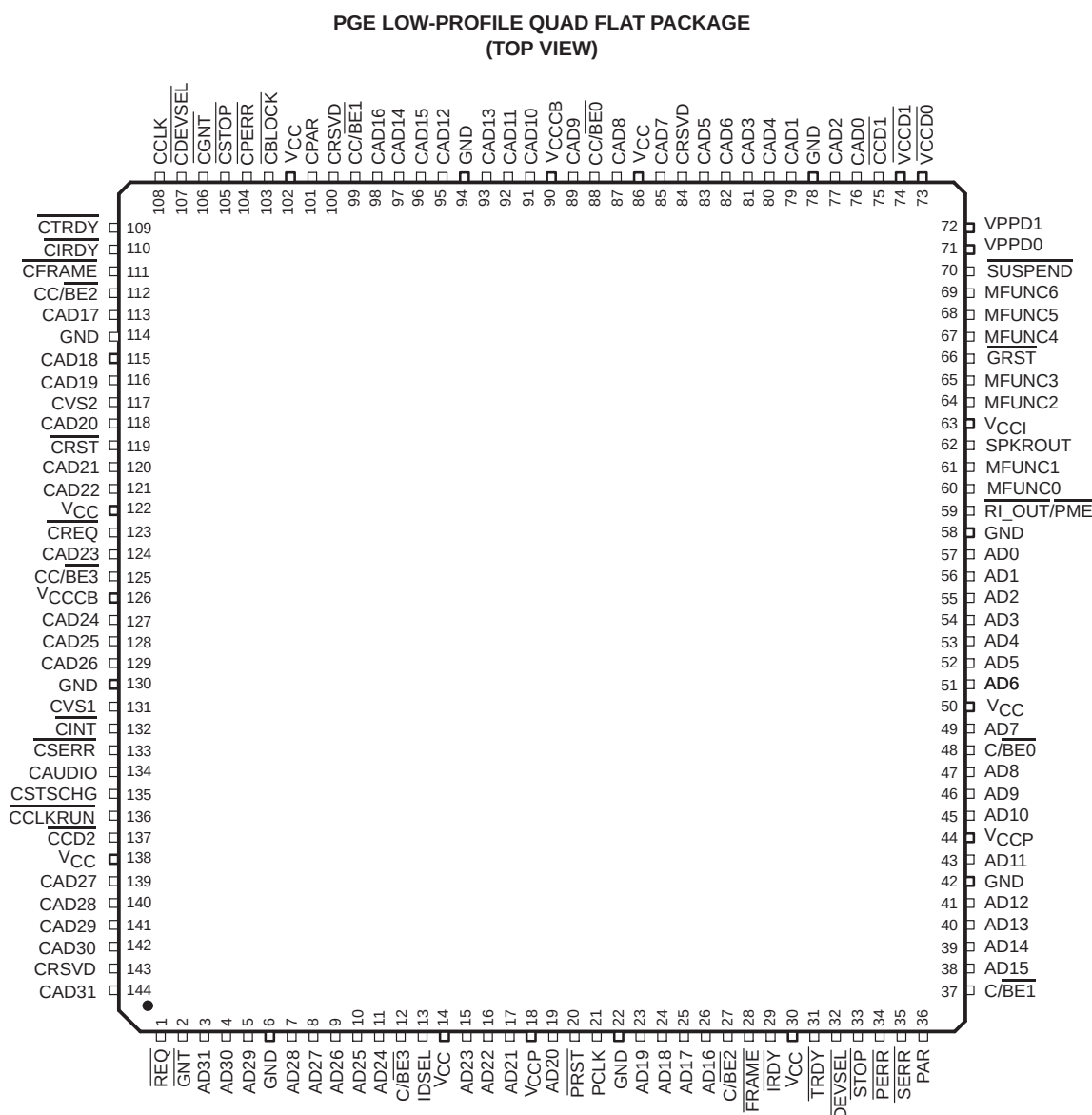
Figure 2–1. PCI-to-CardBus Terminal Diagram
