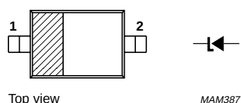
Fig.1 Simplified outline (SOD323) and symbol.
