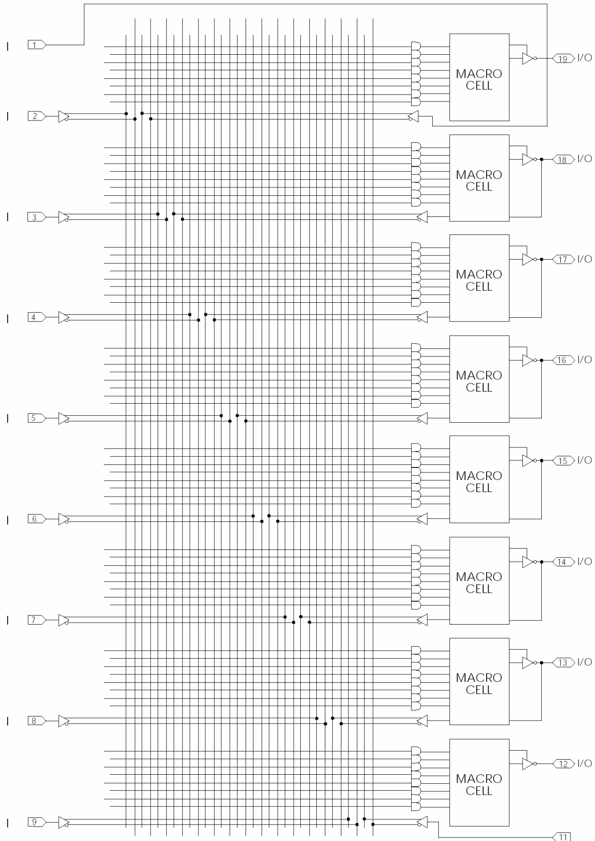
Figure 7 - PEEL TM 16CV8 Logic Array - Complex Mode (see Figure 4 for macrocell details)
