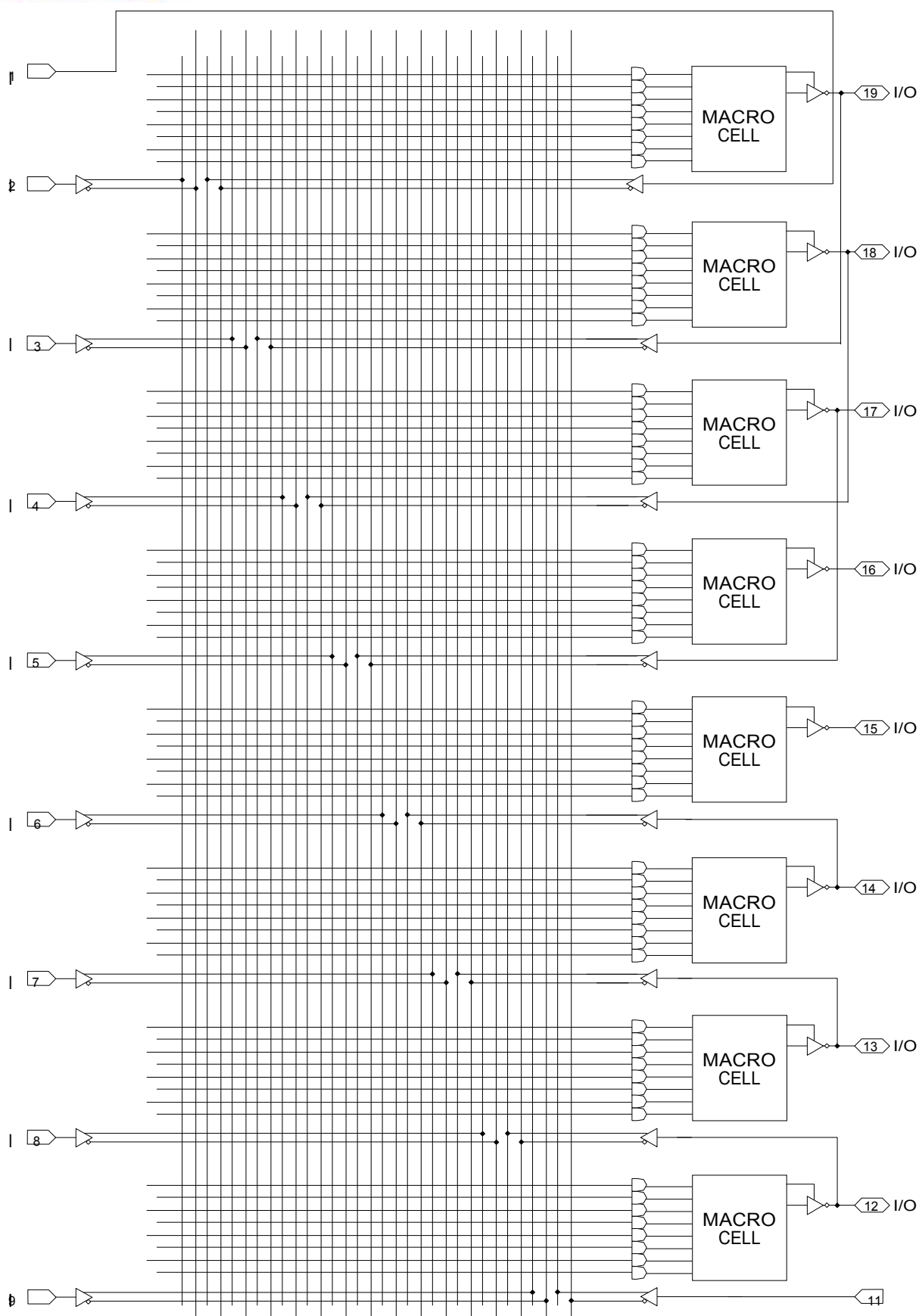
Figure 6 - PEEL TM 16CV8 Logic Array - Simple Mode (see Figure 3 for macrocell details)
