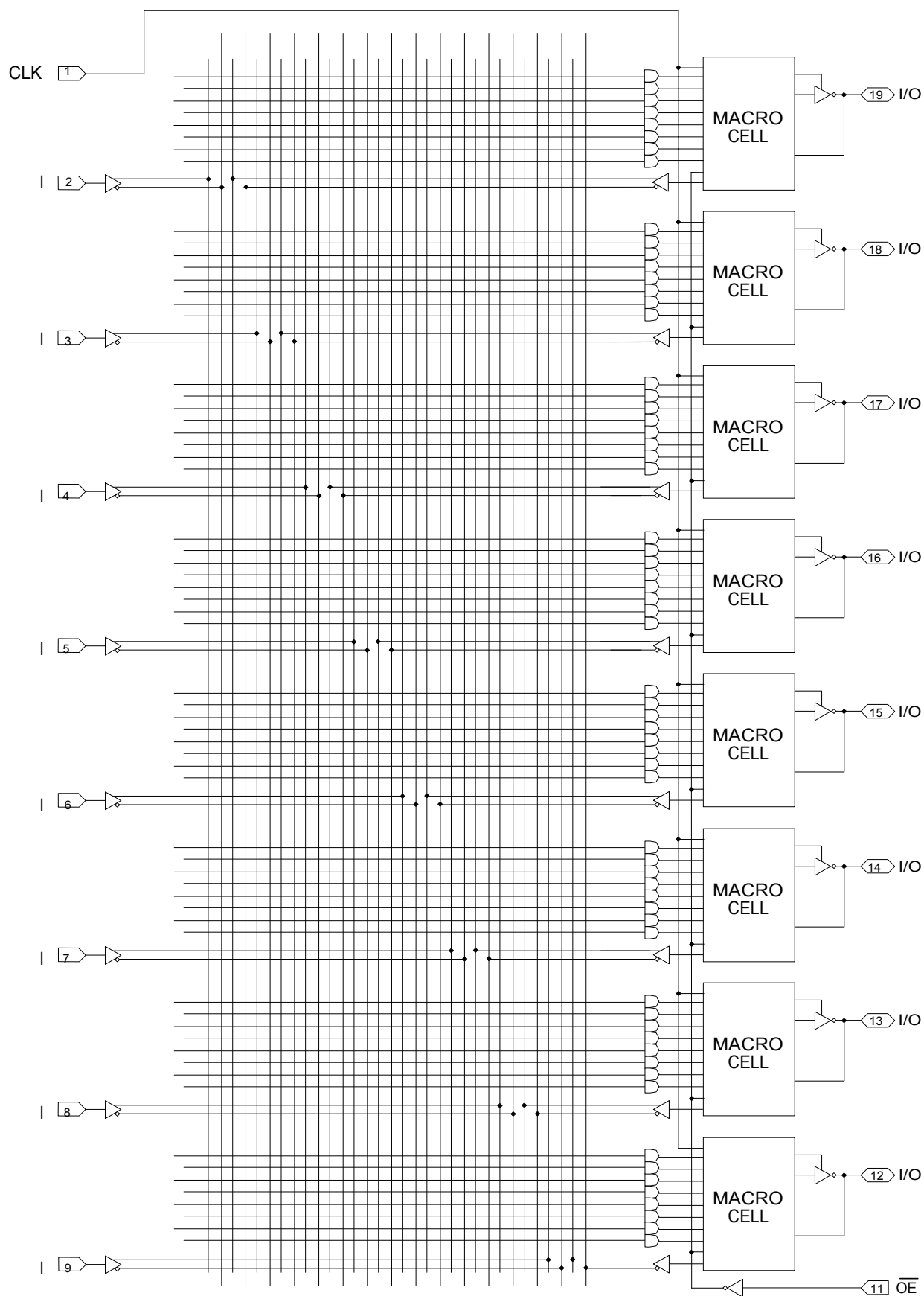
Figure 8 - PEEL TM 16CV8 Logic Array - Registered Mode (see Figure 5 for macrocell details)
