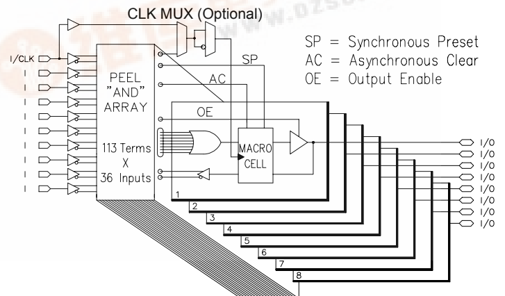
Figure 8 Block Diagram
