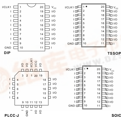
Figure 1 - Pin Configuration
