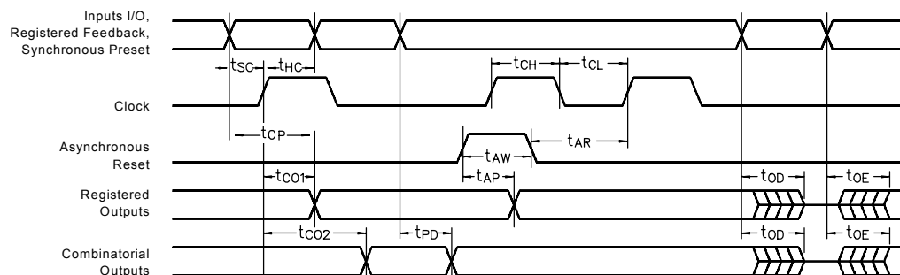
Figure 7 - Switching Waveforms
