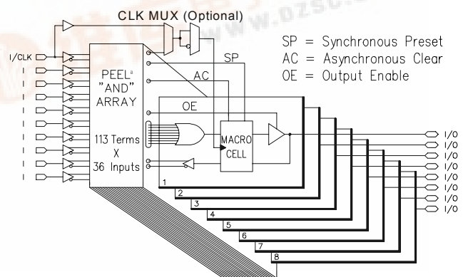
Figure 2 - Block Diagram
