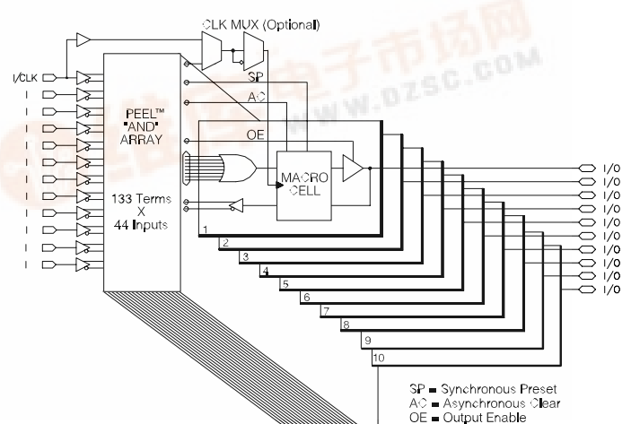
Figure 19 Block Diagram
