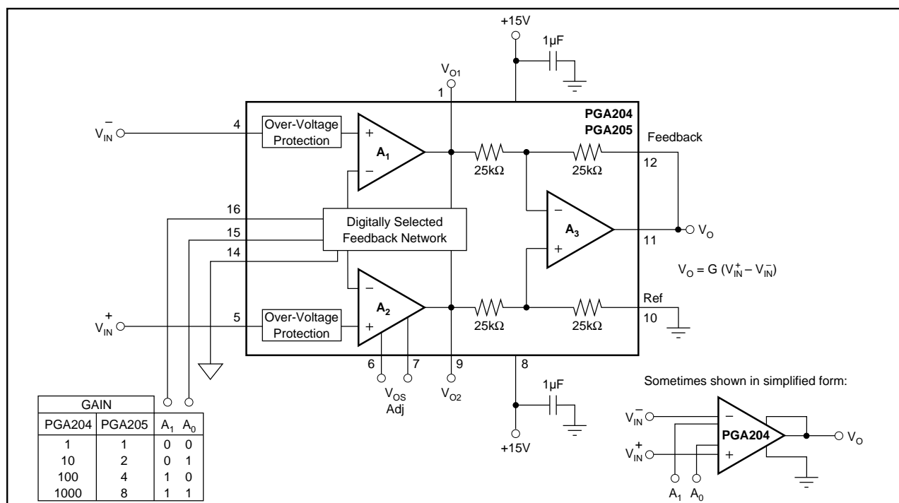
FIGURE 1. Basic Connections.
