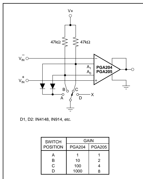
FIGURE 6. Switch-Selected PGIA.
