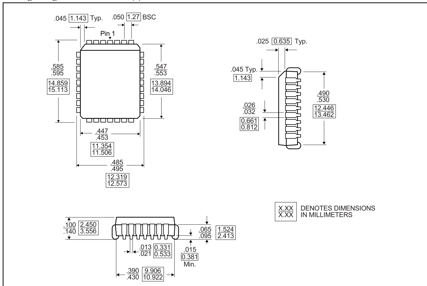
Package Diagram 32-Pin PLCC (J)
