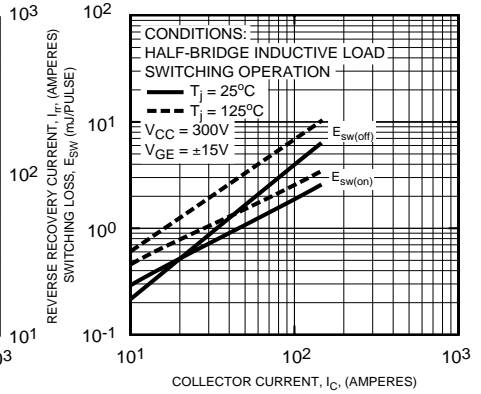
SWITCHING LOSS CHARACTERISTICS
