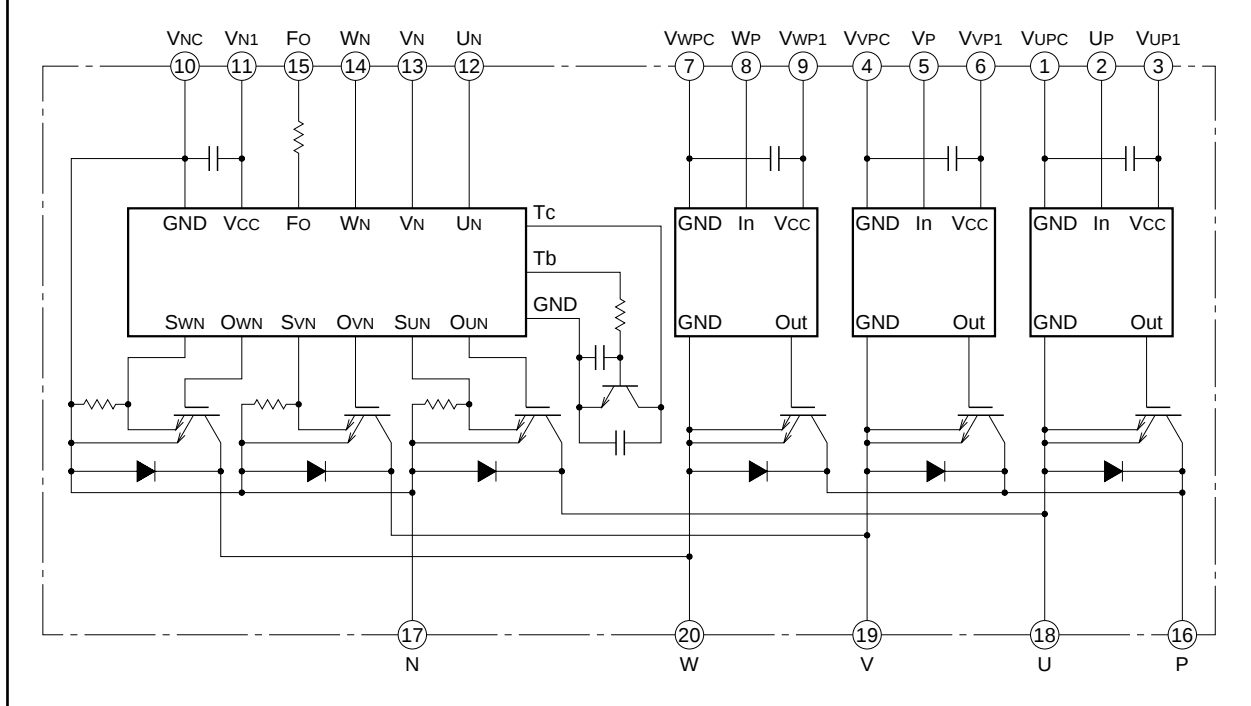
EQUIVALENT CIRCUIT DIAGRAM
