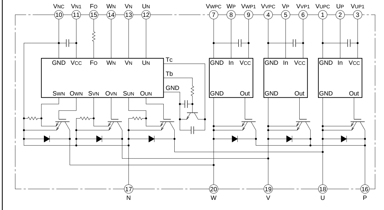
EQUIVALENT CIRCUIT DIAGRAM
