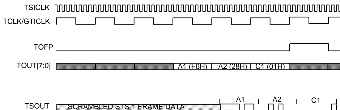
Figure 4 - STS-1 Bit Serial Transmit Frame Pulse and Data Alignment
