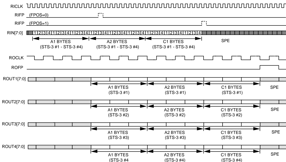
Figure 10 - Byte Interleaved Demultiplex Frame Pulse and Data Alignment
