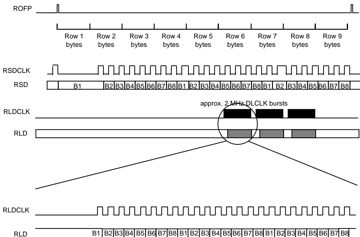
Figure 21 - Receive Data Link Clock and Data Alignment
