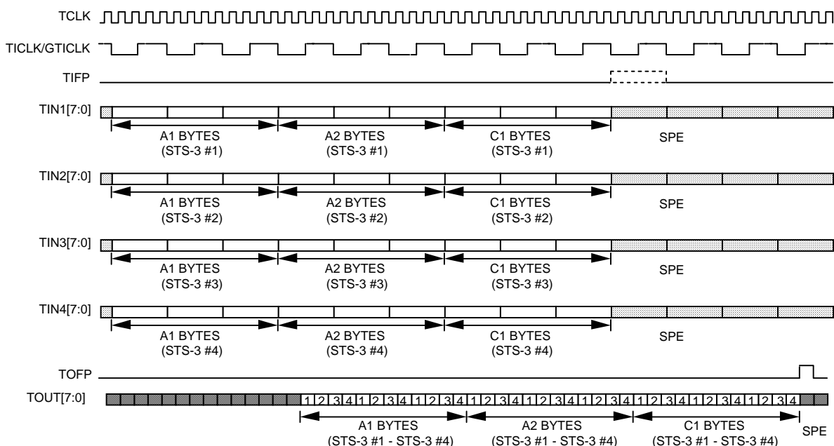
Figure 6 - Byte Interleaved Multiplex Frame Pulse and Data Alignment
