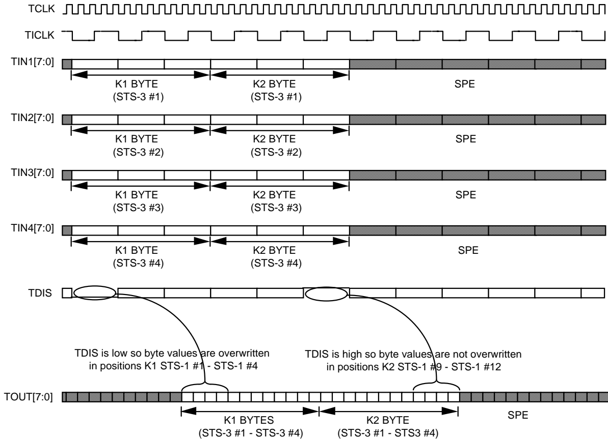
Figure 12 - Transport Overhead Overwrite Enable and Disable with Multiplexing Enabled
