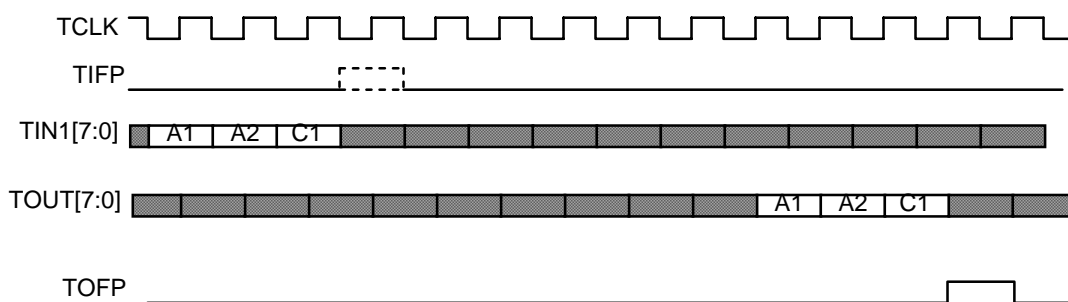
Figure 5 - STS-1 Byte Serial Transmit Frame Pulse and Data Alignment
