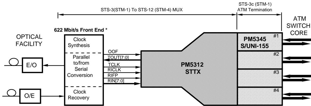
Figure 1 - 622 Mbit/s SONET/SDH Asynchronous Transfer Mode Multiplexer
