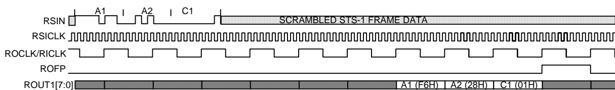
Figure 8 - STS-1 Bit Serial Receive Frame Pulse and Data Alignment
