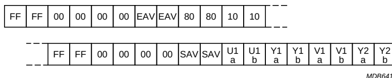
Fig 7. YUV 4:2:2 Interleaved
