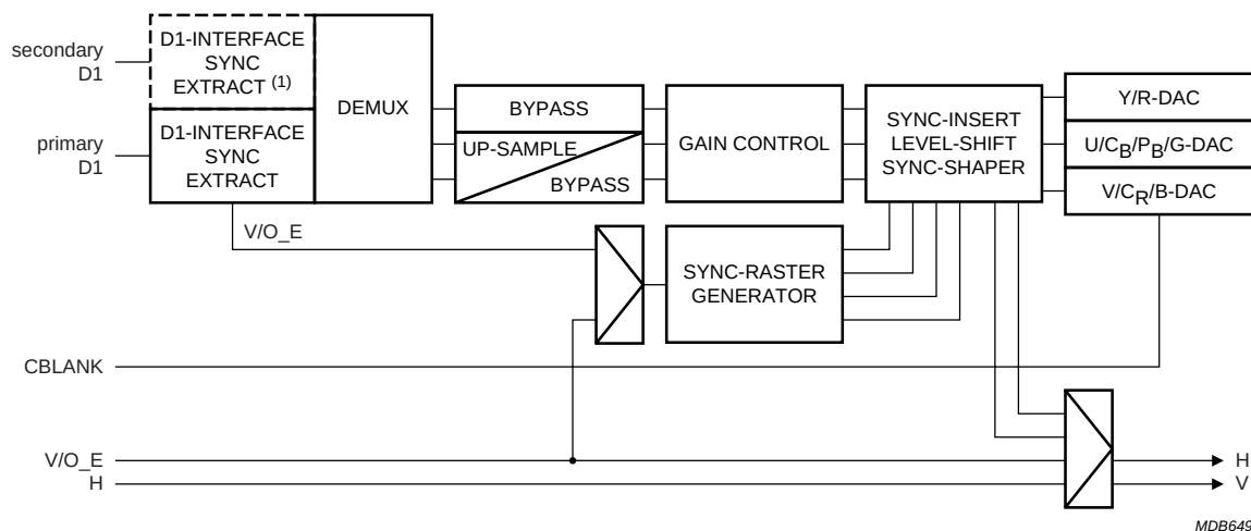
Fig 15. Primary display pipe
