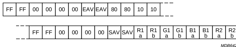
Fig 8. RGB 4:4:4 Interleaved
