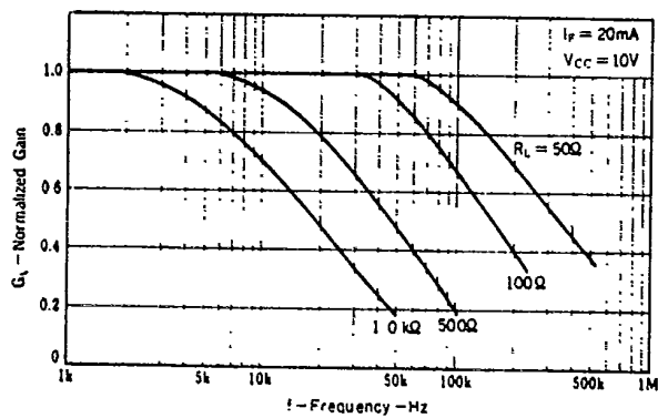
FREQUENCY RESPONSE
