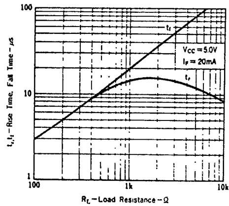
SWITCHING TIME vs. LOAD RESISTANCE
