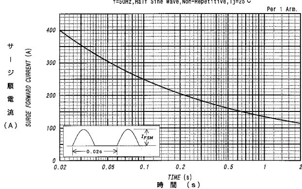
サージ順電流定格 SURGE CURRENT RATINGS f=50\text{Hz} , Half Sine Wave, Non-Repetitive, T_j=25^\circ\text{C}
