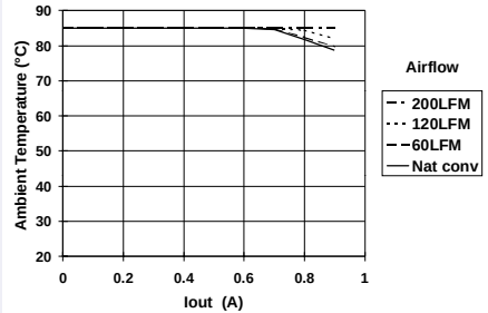
Safe Operating Area @ V_{in} = 48\text{V} (Note B)
