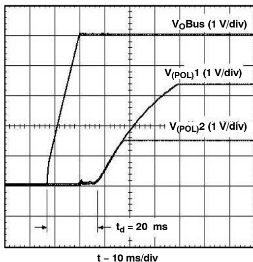
Figure 29. Power-Up Waveform
