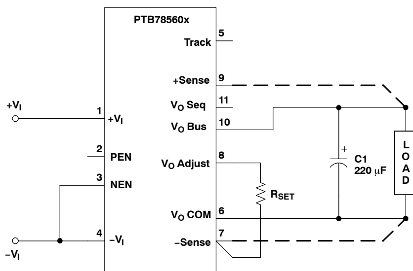
Figure 31. Stand-Alone Configuration
