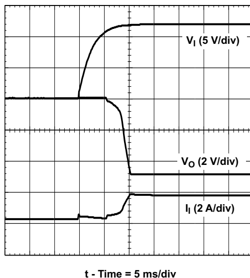
Figure 18. Power-Up Waveforms
