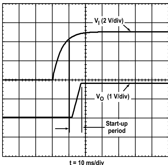
Figure 14. PTV05010W Start-Up
