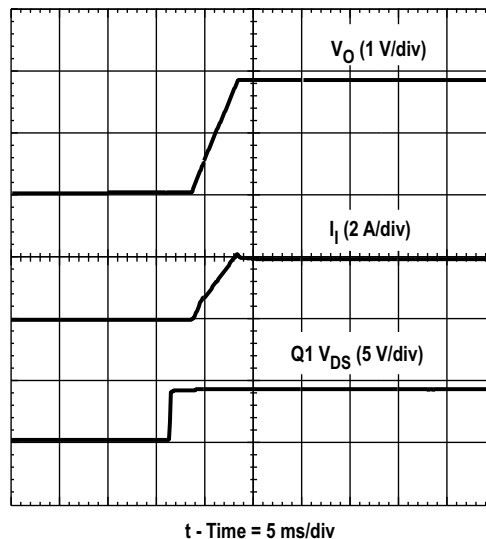
Figure 10. Inhibit Waveform
