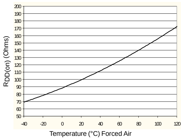
Figure 3. Typical On-Resistance
