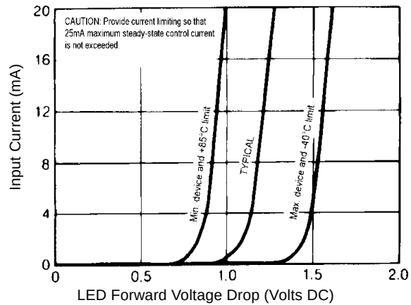
Figure 5. Input Characteristics (Current Controlled)
