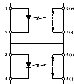
Connection Diagram
