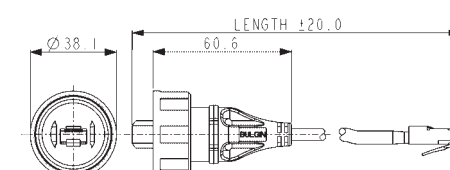
PX0837 - single ended
