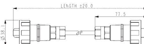
PX0832 - double ended
