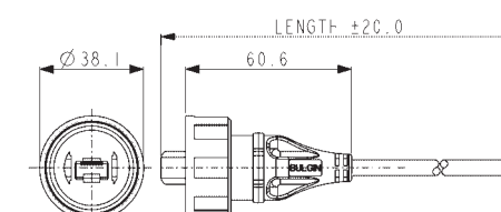
PX0836 - wire ended
