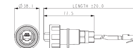
PX0831 - single ended
