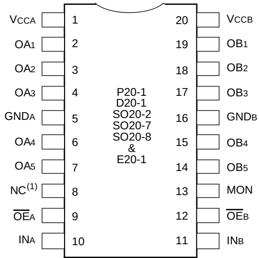
DIP/SSOP/SSOP/QSOP/CERPACK TOP VIEW
