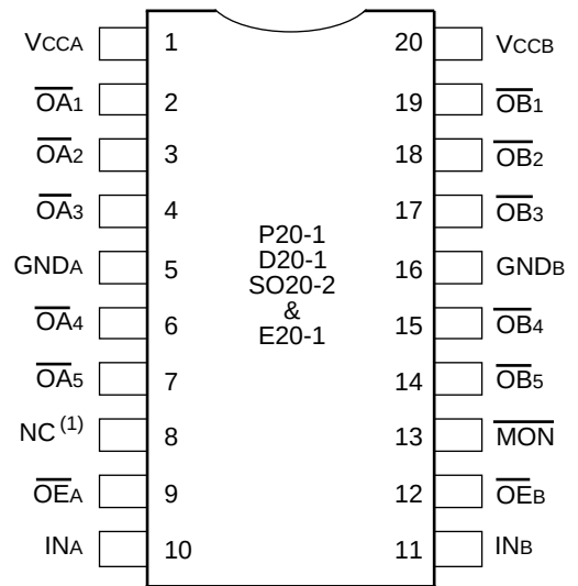
DIP/SSOP/CERPACK TOP VIEW
