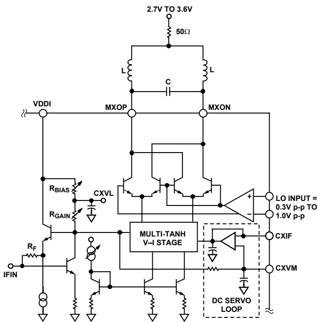
Figure 43. Simplified Schematic of AD9864's LNA/Mixer
