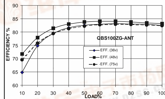
Efficiency vs. Load (48V Input)
