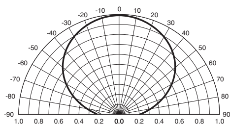
Fig.3 Radiation Diagram
