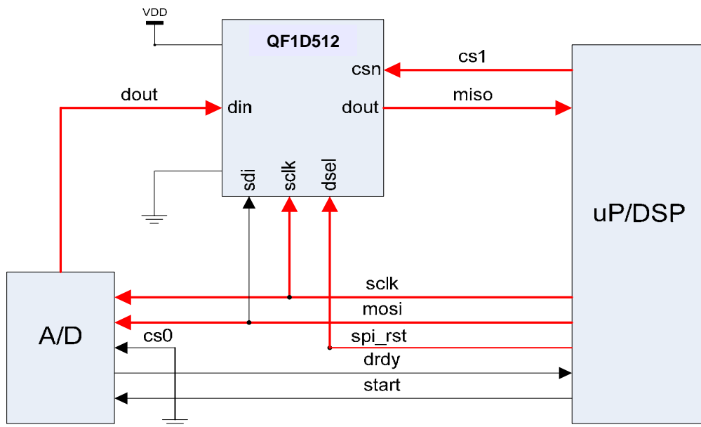
Figure 8 : Inline Continuous SPI Mode
