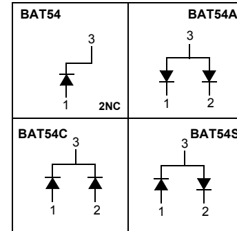
Connection Diagram
