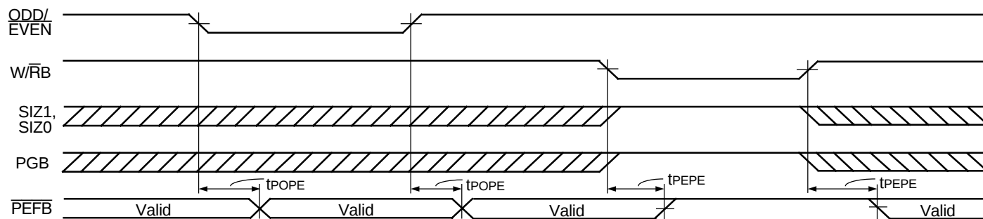
Figure 17. ODD/EVEN, W/RB, SIZ1, SIZ0, and PGB to \overline{PEFB} Timing
