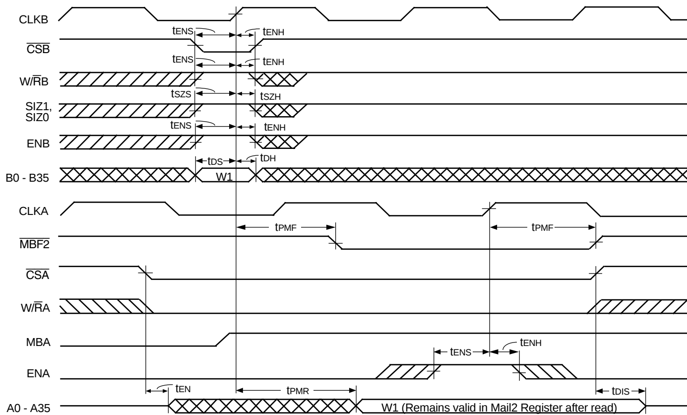
Figure 15. Timing for Mail2 Register and \overline{MBF2} Flag
