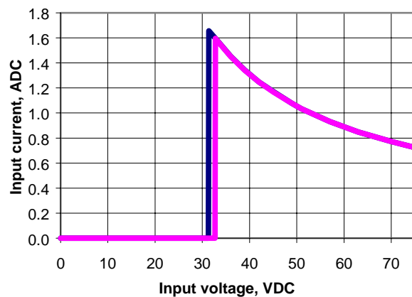
Fig. 5 QLS30ZA Input Characteristic
