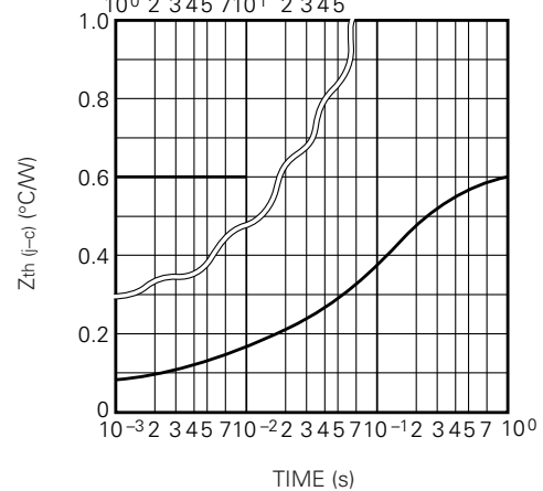
TRANSIENT THERMAL IMPEDANCE CHARACTERISTIC
