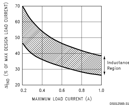
FIGURE 16. ( \Delta I_L ) Peak-to-Peak Inductor Ripple Current (as a Percentage of the Load Current) vs Load Current
