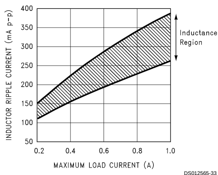
FIGURE 18. Peak-to-Peak Inductor Ripple Current vs Load Current
