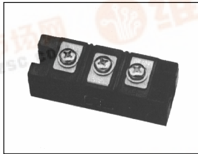
QR_0610T30 Fast Recovery Diode Module 100 Amperes / 600 Volts
