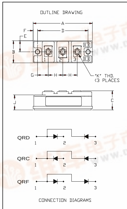
QR_0610T30 Fast Recovery Diode Module 100 Amperes / 600 Volts
