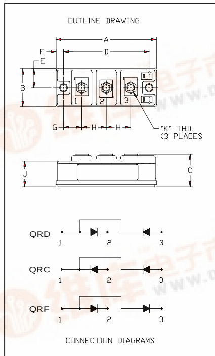
QR_0630T30 Fast Recovery Diode Module 300 Amperes / 600 Volts
