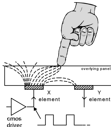
Figure 1-3 Fields With a Conductive Film
