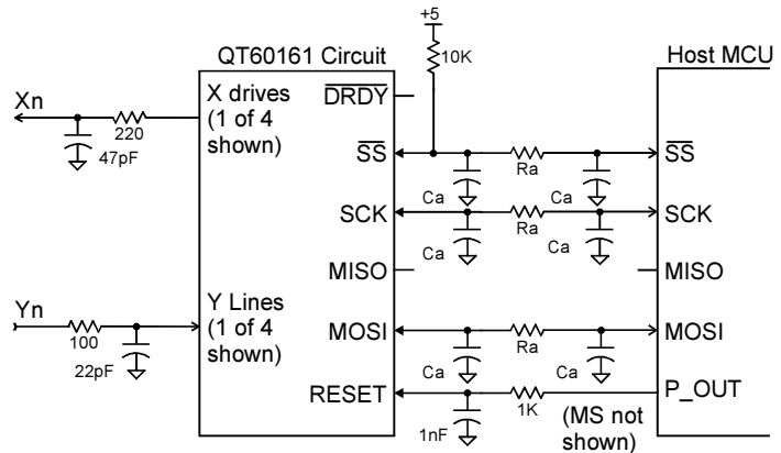
Figure 4-7 Filtering; SPI Master-Slave Connections
