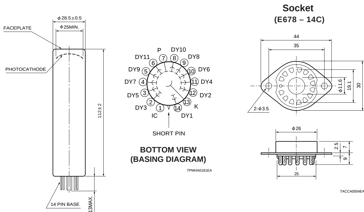
Figure 2: Dimensional Outline and Basing Diagram (Unit : mm)
